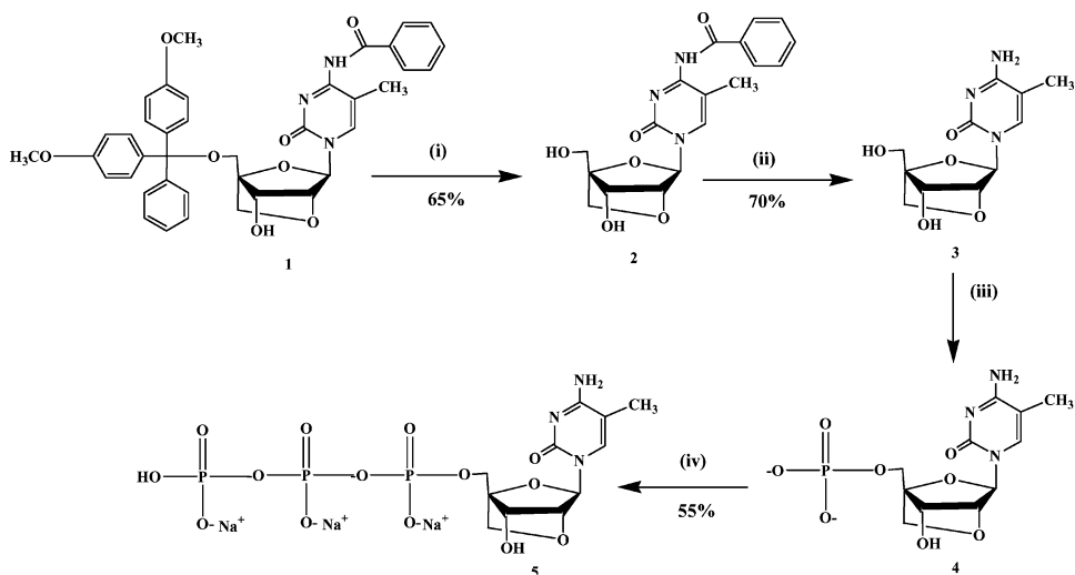
SCHEME 1 Chemical synthesis of locMeCytidine-5'-triphosphate (1) 3% TCA in DCM, r.t. 2 hours, 65%; (2) \text{NH}_4\text{OH} /ACN, 3:1, 55°C, 16 hours, 70%; (3) [\text{MeO}]_3\text{PO}/\text{POCl}_3 , 0°C, 3 hours; (4) [\text{Bu}_3\text{NH}^+]_4\text{P}_2\text{O}_7^{4-} , DMF, 0°C, 1 minutes, 0.1 M TEAB, 75 mL, r.t., 5 hours, 55%.
