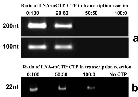
FIGURE 1 Electrophoresis pictures show the transcription efficiency of LNA-mCTP. In the reaction, when the ratio of LNA-mCTP to normal CTP reached 50%, 100- and 200-nt transcripts could not be synthesized (a). 100- or 200-nt transcripts were transcribed only when LNA-mCTP accounted for 20% of the CTP source in the reaction. However, the yield of 100- and 200-nt RNAs were much less than when transcribed with normal CTP only (a). In contrast, 22-nt transcripts were successfully generated even if LNA-mCTP accounted for 50 or 100% of the CTP sources in the reaction (b), but the yield of the transcripts was greatly reduced as compared to that without LNA-mCTP. No RNA product can be made when the reaction is lacking any form of CTP (no CTP data in lane 6).
